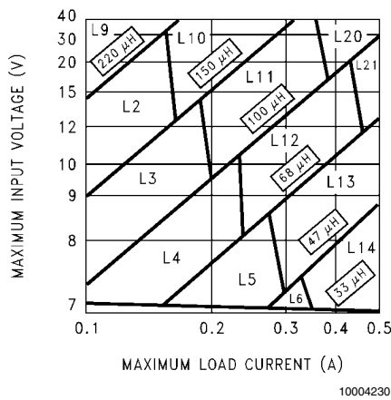
FIGURE 5. LM2671-5.0
